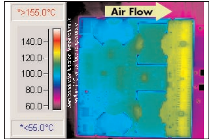
Figure 8: Thermal plot of converter at 52 amp load current with 55°C air flowing at the rate of 200 LFM. Air is flowing across the converter from input to output (nominal input voltage).
