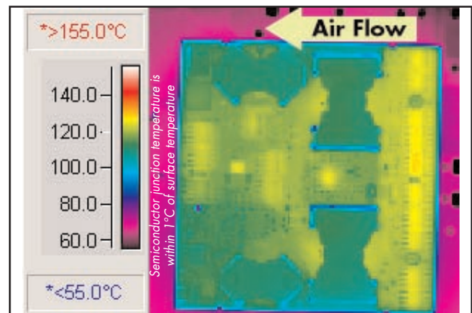
Figure 6: Thermal plot of converter at 54 amp load current with 55°C air flowing at the rate of 200 LFM. Air is flowing across the converter from output to input (nominal input voltage).
